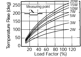
Temperature Rise (ref.)
