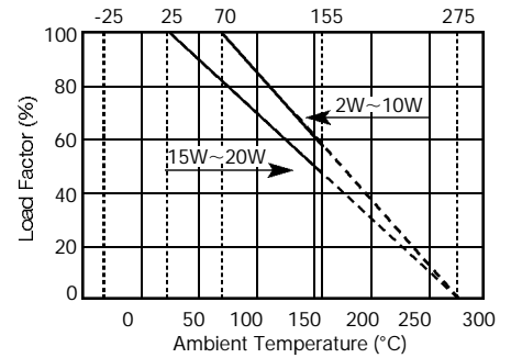
Derating Curve
