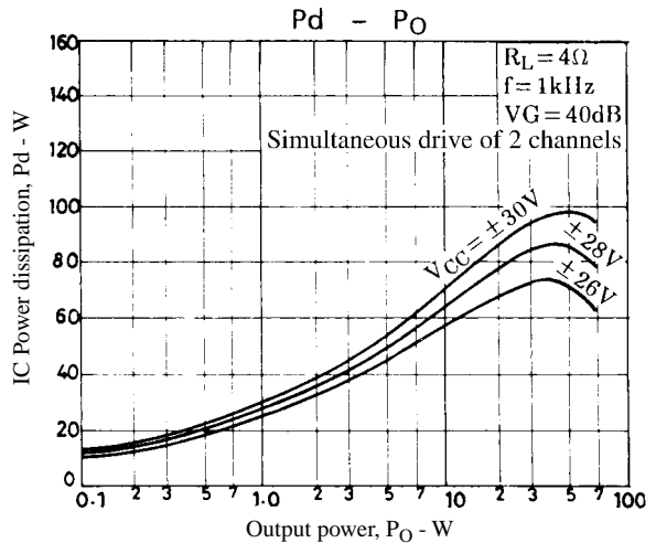
Figure 2. STK4171V Pd - P O (R L = 4Ω)
